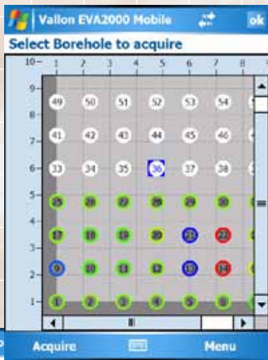
borehole plan
